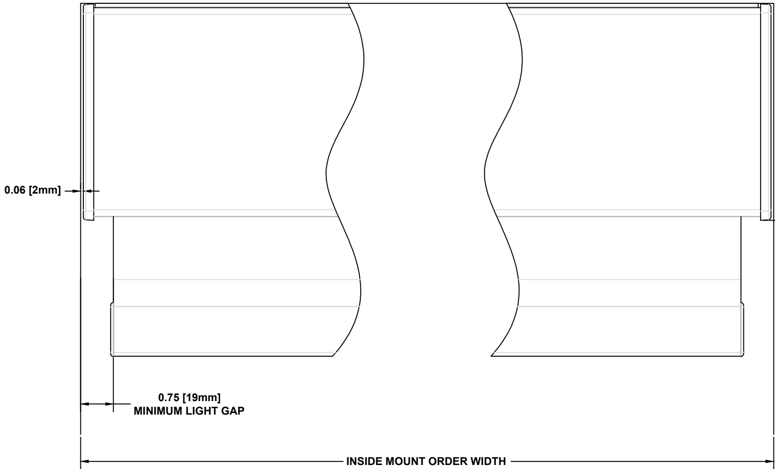
TYPICAL ELEVATION (ROOM VIEW)
