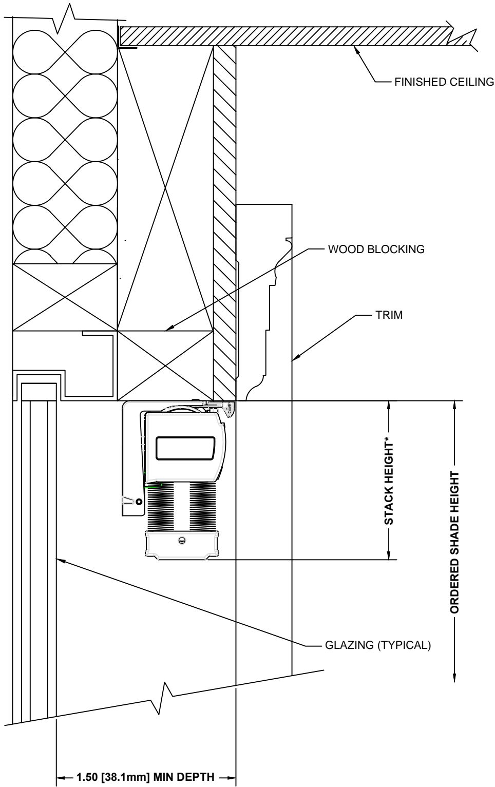
TYPICAL SECTION
