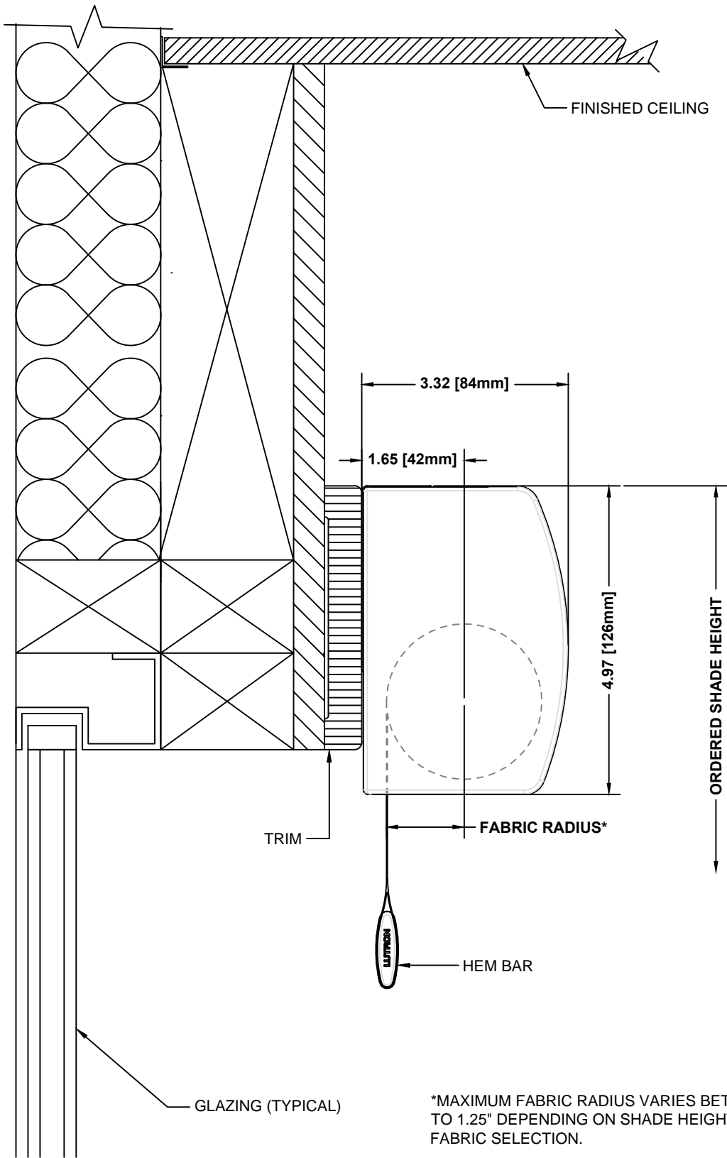
TYPICAL SECTION
