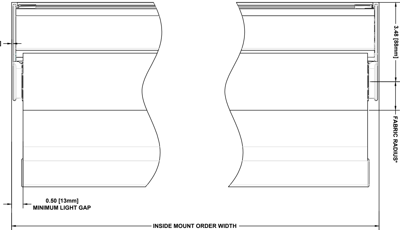
TYPICAL ELEVATION (ROOM VIEW)
