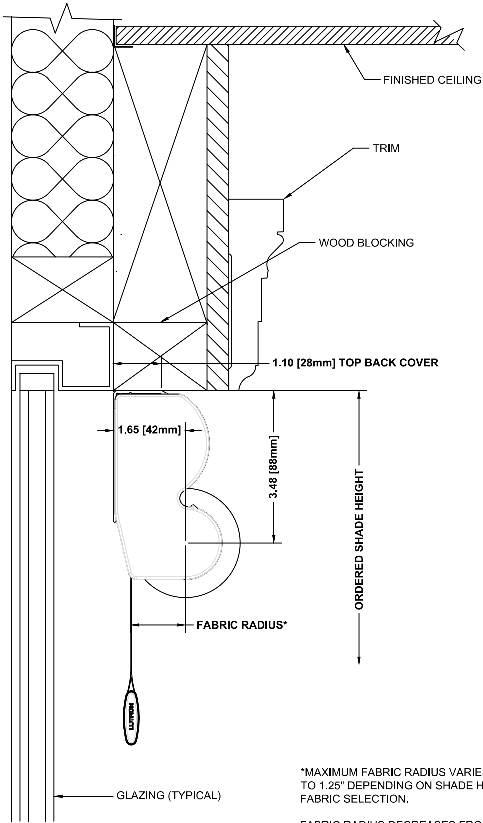
TYPICAL SECTION
