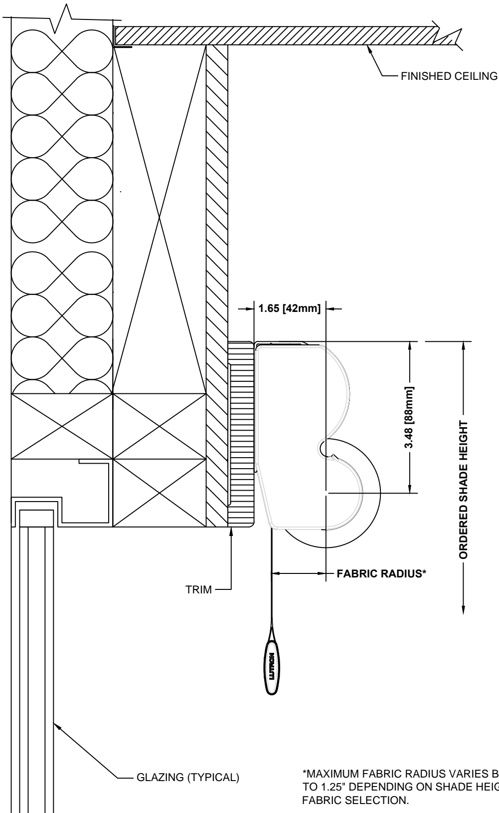
TYPICAL SECTION
