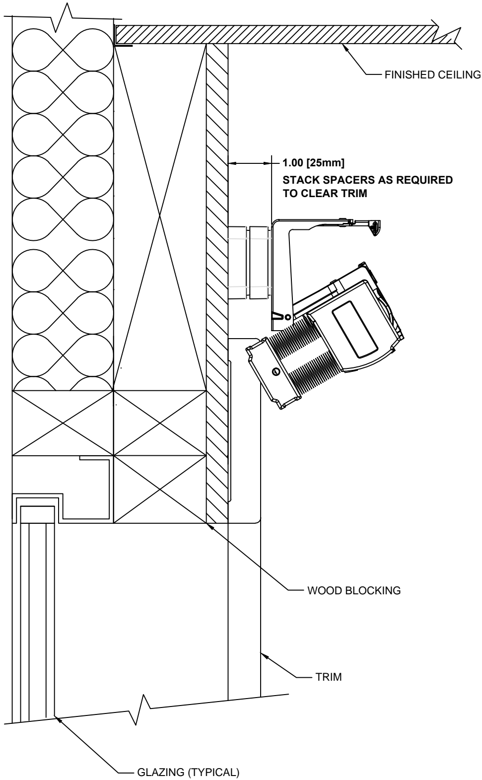
TYPICAL SECTION
