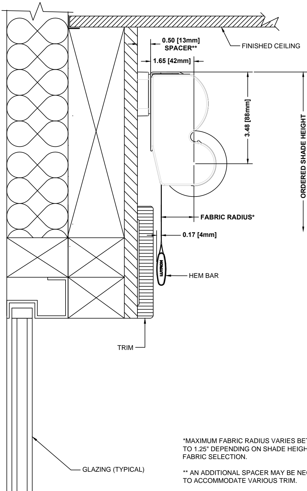
TYPICAL SECTION
