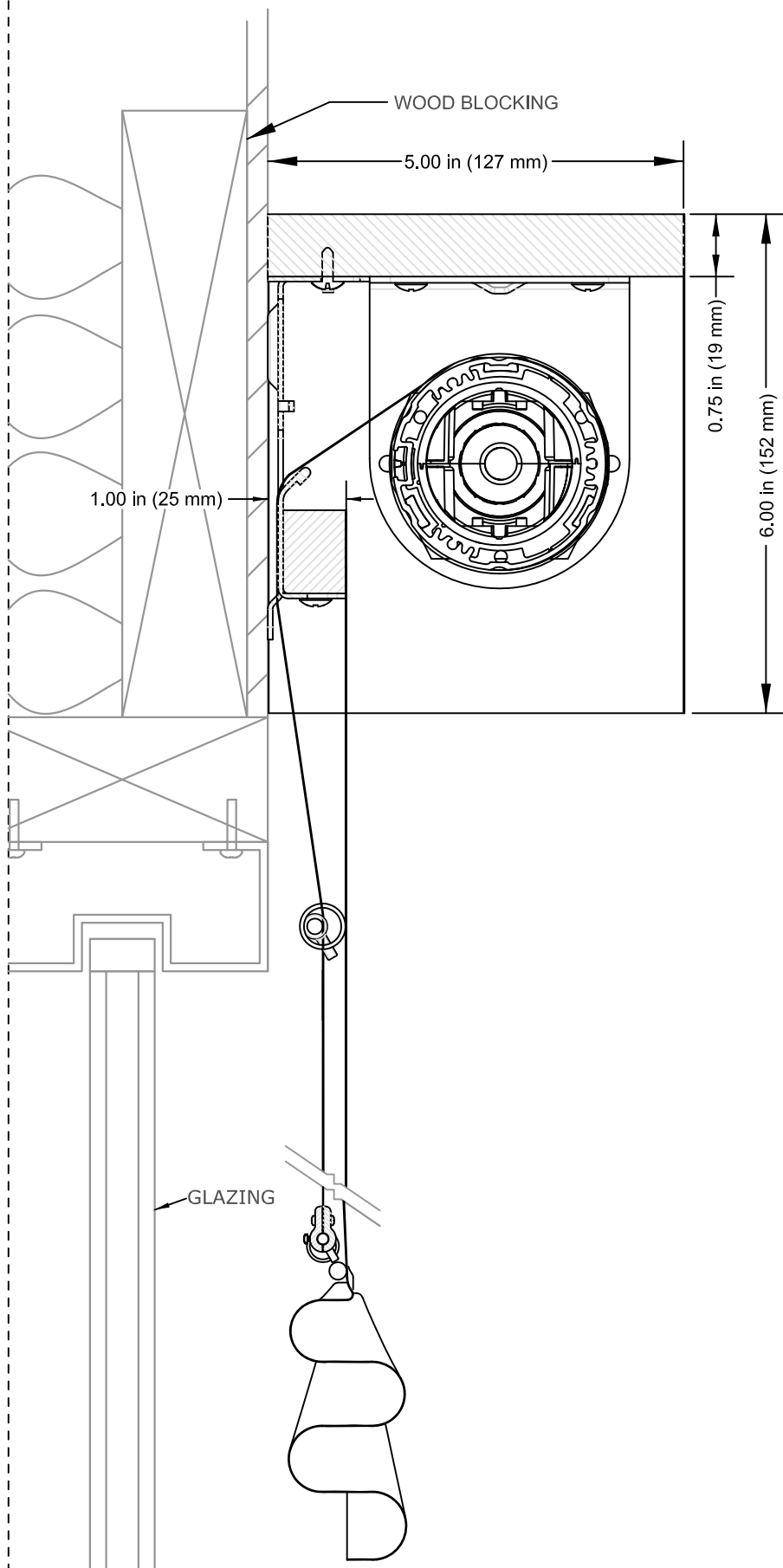
FRONT CONTROL - TYPICAL SECTION
