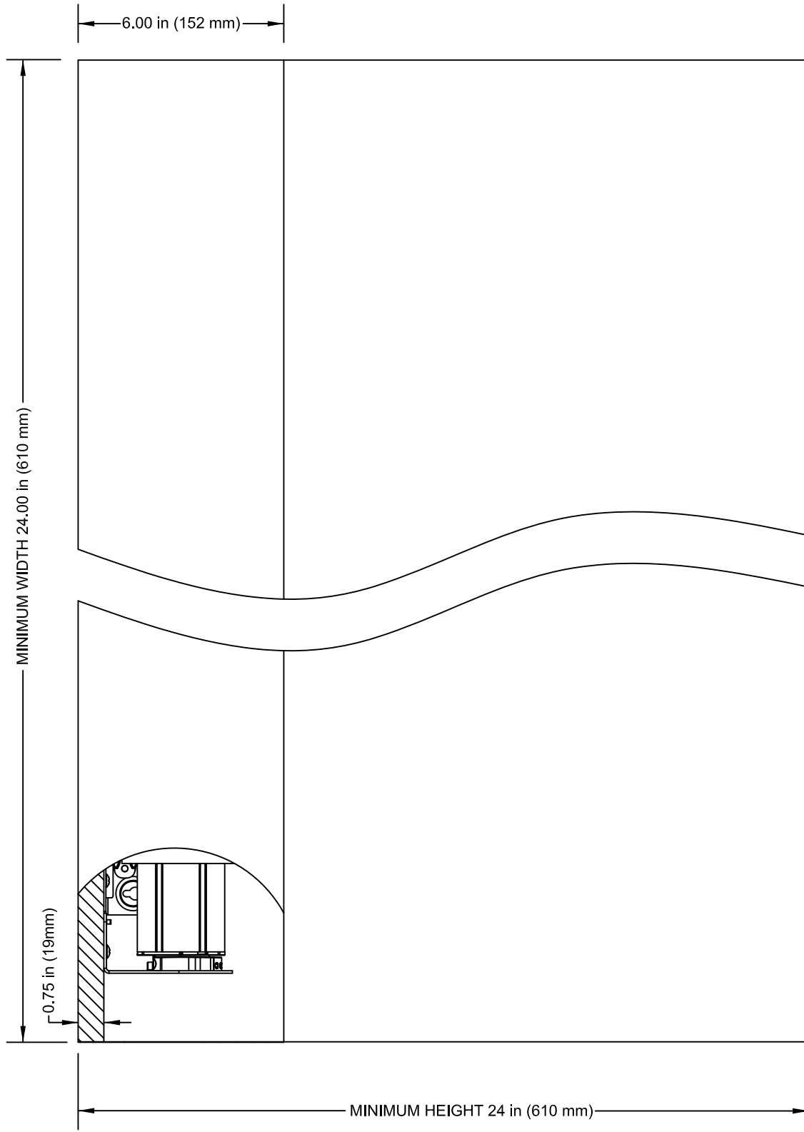
TYPICAL ELEVATION (ROOM VIEW)
