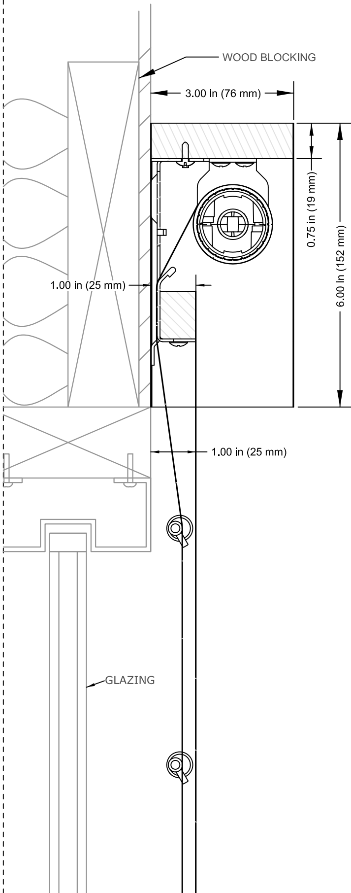
1 FRONT CONTROL - TYPICAL SECTION
