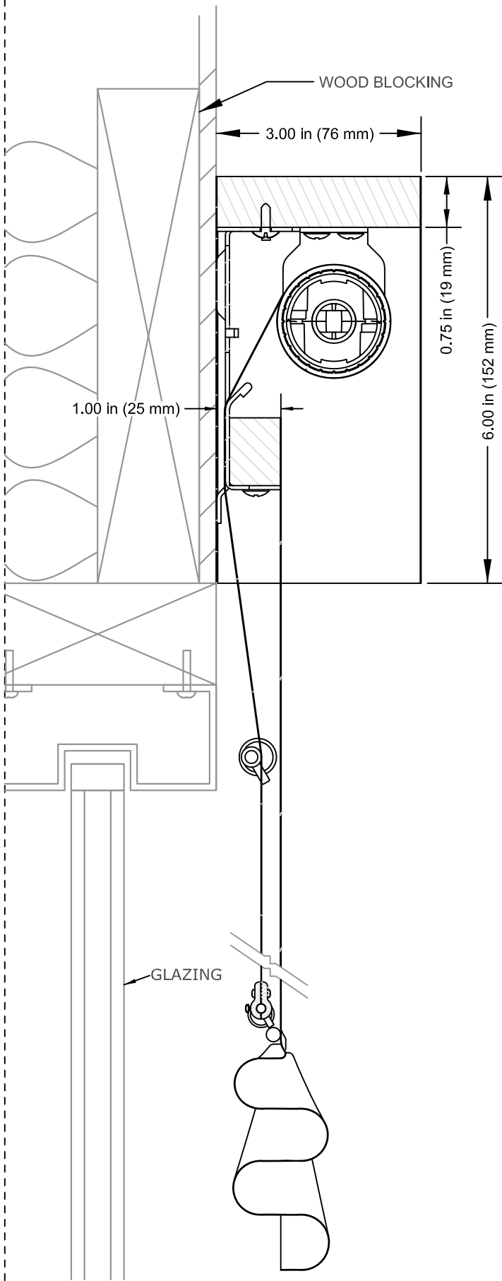
1 FRONT CONTROL - TYPICAL SECTION SCALE: 1/2
