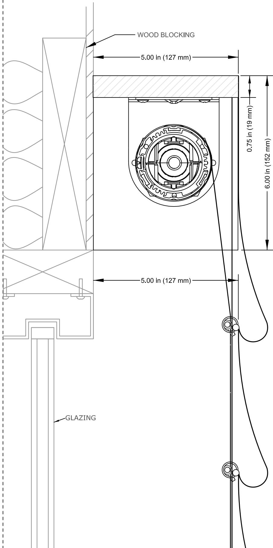
1 BACK CONTROL - TYPICAL SECTION
