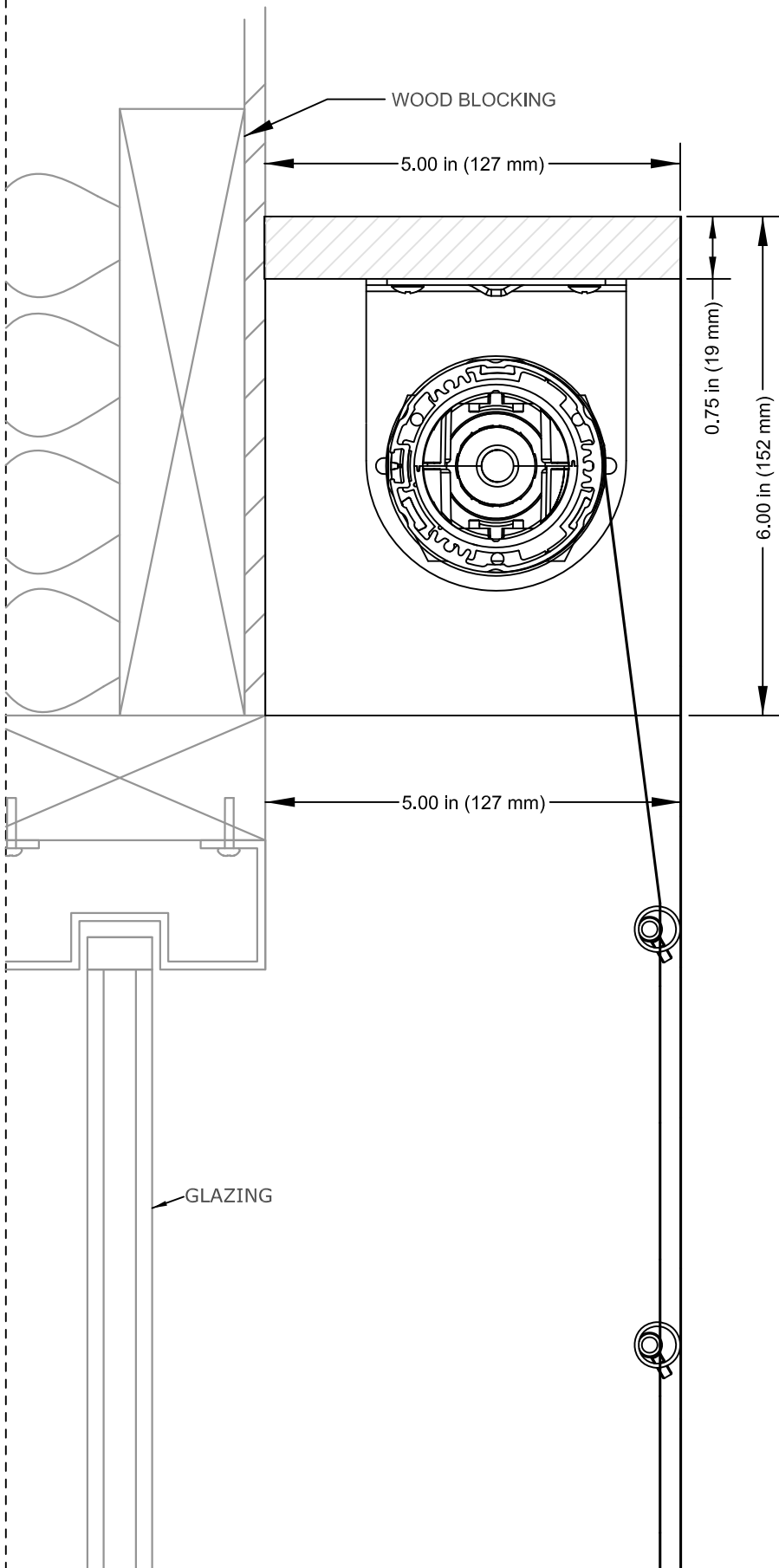
BACK CONTROL - TYPICAL SECTION
