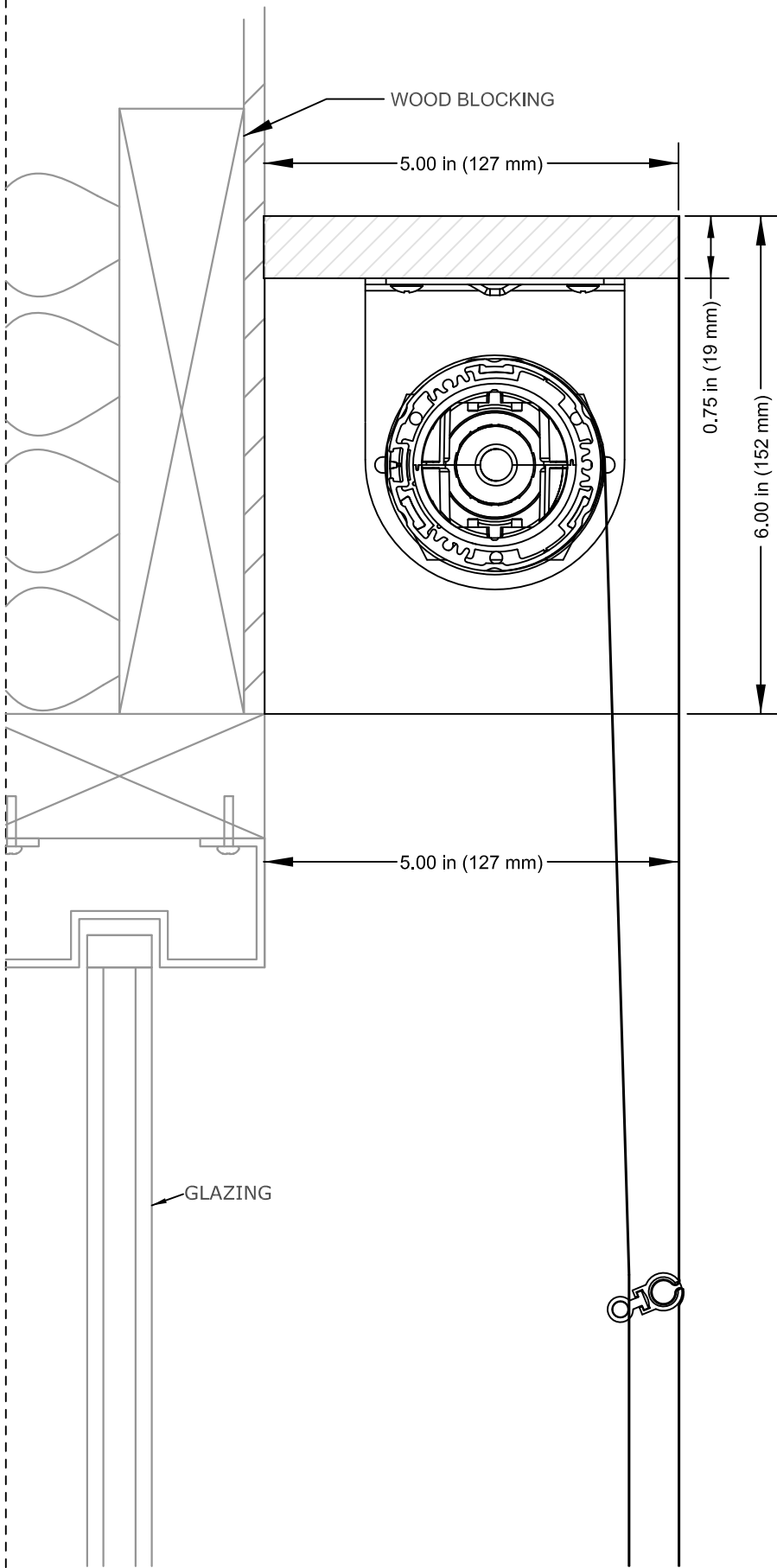
1 BACK CONTROL - TYPICAL SECTION
