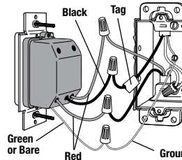
Green or Bare Red Ground
