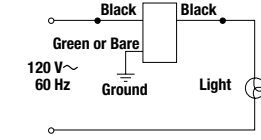
Green or Bare Ground
