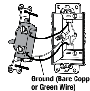
Ground (Bare Copper or Green Wire)
