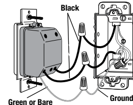
Green or Bare Ground
