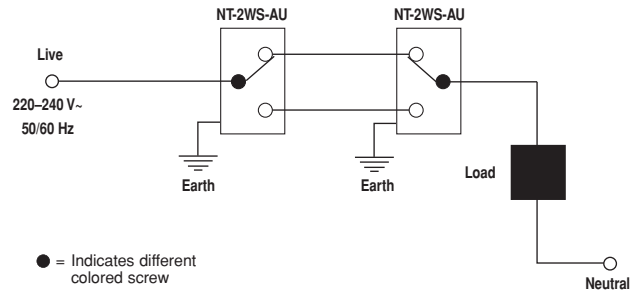
Figure B. Wiring Diagram - 2-Way
