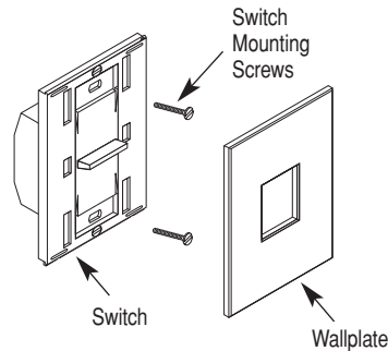
Figure C. Mounting Diagram
