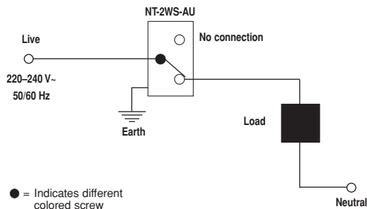
Figure A. Wiring Diagram - Single-Pole
