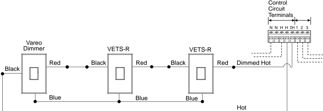
Diagram 10: Vareo Dimmer (Three location)
