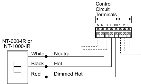
Diagram 11: Nova T* Infrared Dimmer
