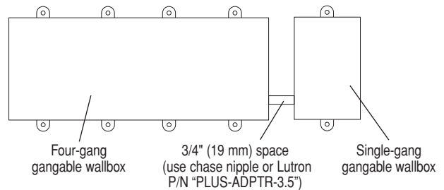
Figure B. Wallbox Ganging
