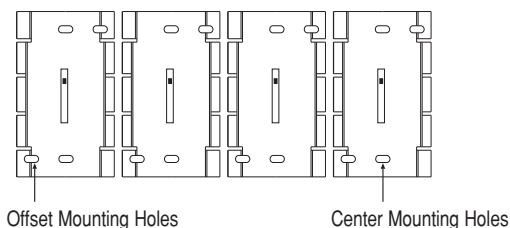
Figure C. Front View - Four-Gang Installation
