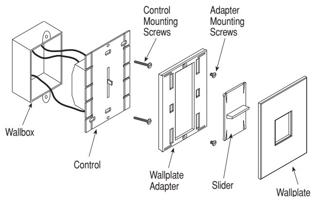
Figure A. Control Mounting
