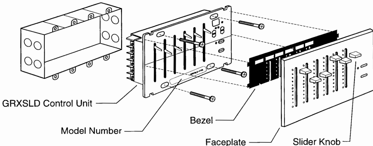
Mounting Diagram
