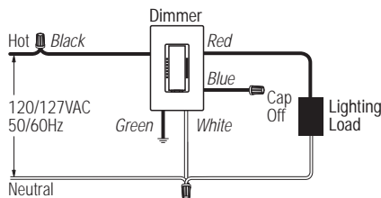
Single-Location Installation
