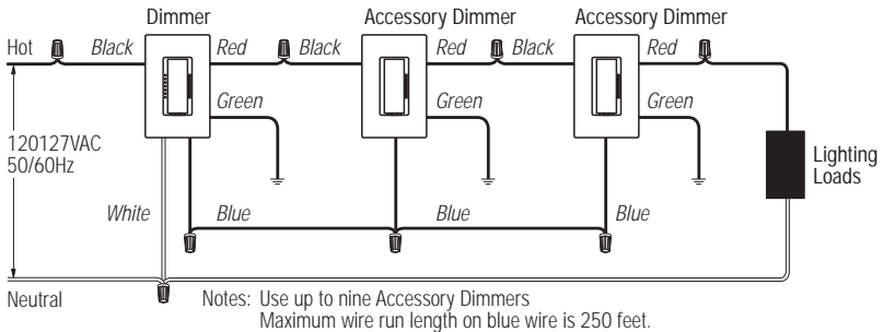
Multi-location Installation
