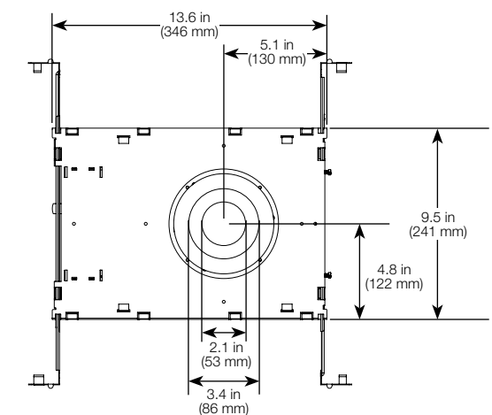
Bottom view (Trimmed)
