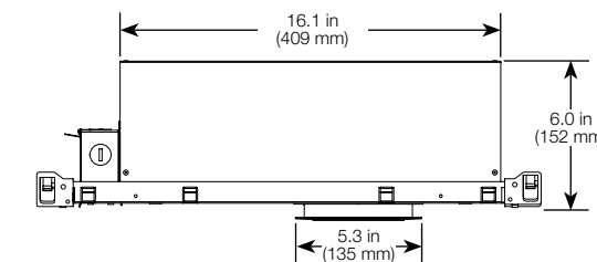
Side view (Trimless)
