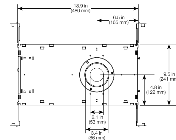
Bottom view (Trimless)
