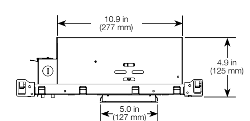
Side view (Trimmed)
