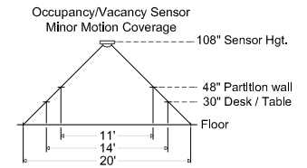
SENSOR COVERAGE - N.T.S. TYPICAL OFFICE FURNITURE HEIGHTS
