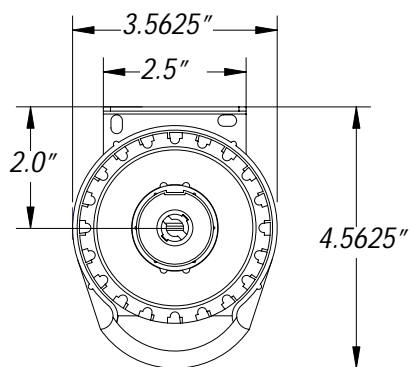
Ceiling Mount
