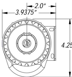
Wall Mount
