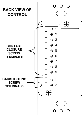
Control Schematic
