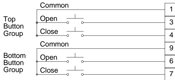
Control Schematic
