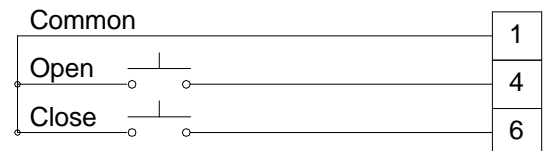
Control Schematic
