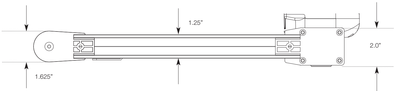
One-Way Draw Top View
