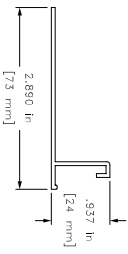
3 in [76 mm] POCKET FLAP (OPTIONAL)
