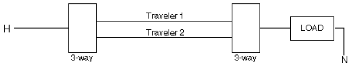
Existing 3-way switch wiring
