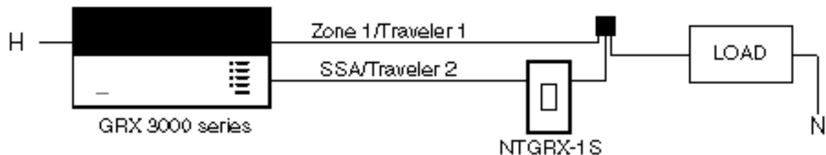
Retrofit: GRX-3000 on line side
