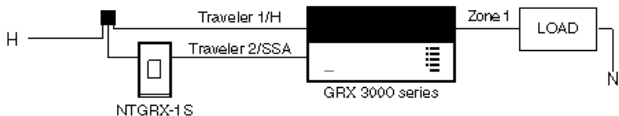
Retrofit: GRX-3000 on load side
