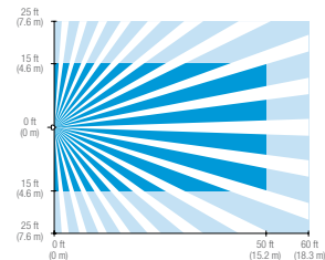
Wall mount (LRF2-OWLB-P-WH)
