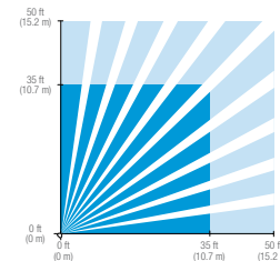
Corner mount (LRF2-OKLB-P-WH)
