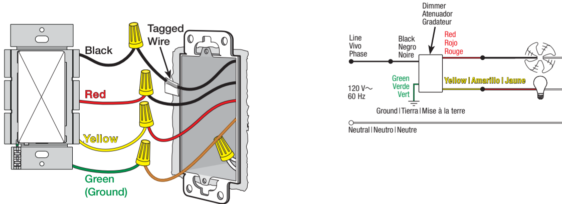
Image #31 — Fan Control with One Black Wire, One Red Wire and One Yellow Wire in a Single Pole Application
