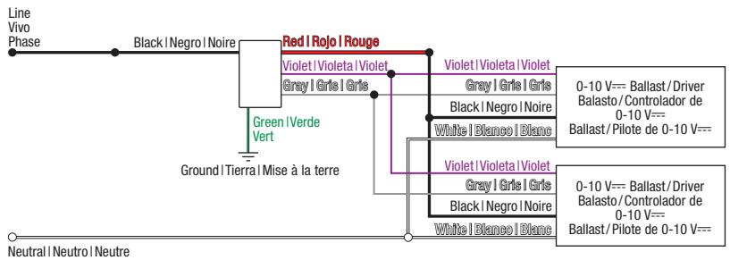
Image #66 — Dimmer with One Black Wire, One Red Wire, One Violet Wire, and One Gray Wire in a Single Pole Application (without a power pack)
