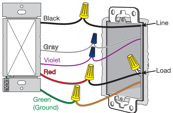
Image #66 — Dimmer with One Black Wire, One Red Wire, One Violet Wire, and One Gray Wire in a Single Pole Application (without a power pack)
