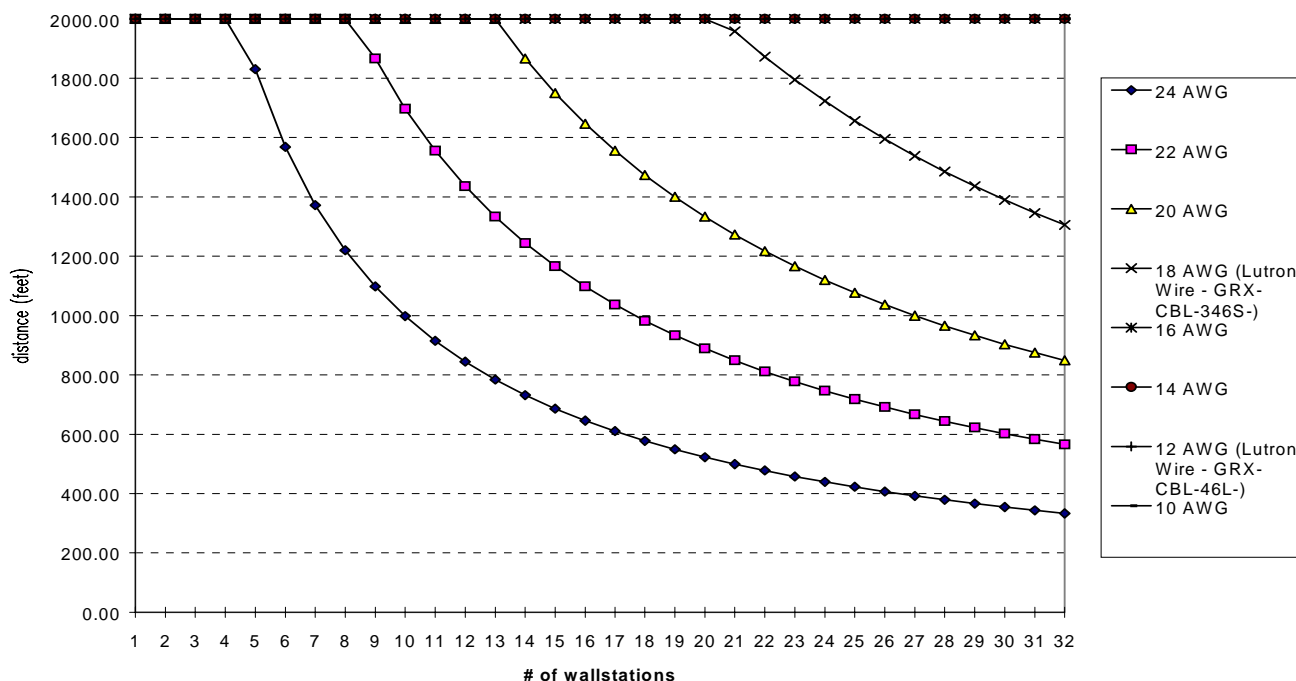
GRAFIK 6000 33VDC power supply (provided in all G6000 panels) Wallstations evenly spaced on link
